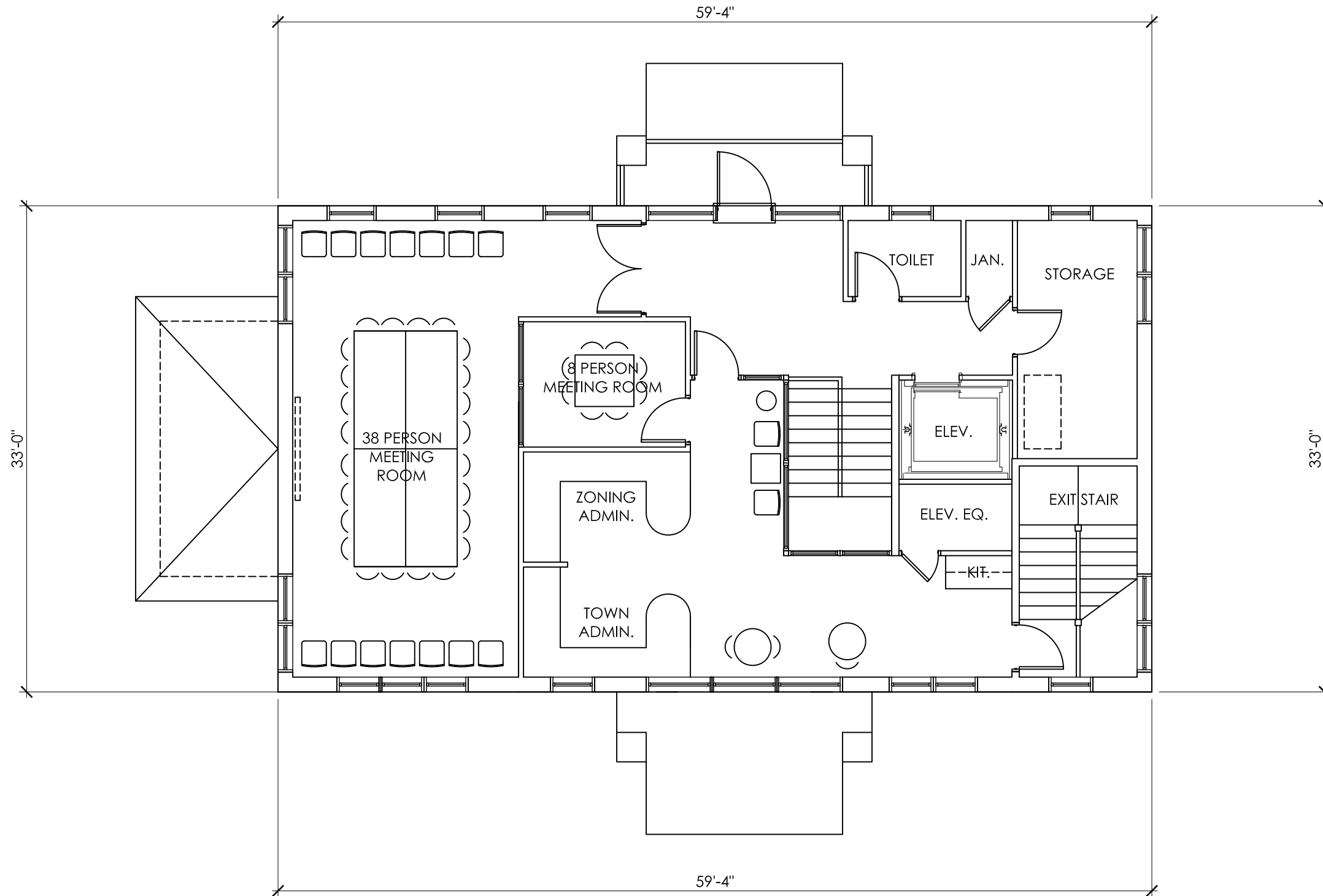
PROPOSED 2nd FLOOR PLAN 1762 GSF
