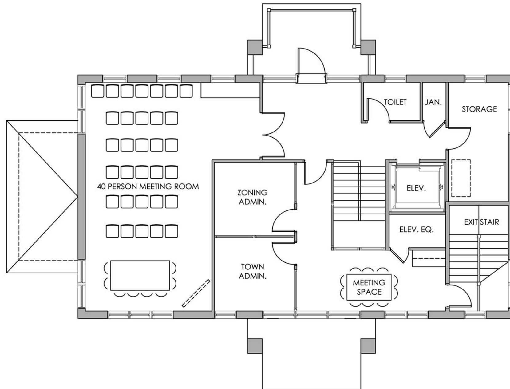
PROPOSED 2nd FLOOR PLAN 1762 GSF
