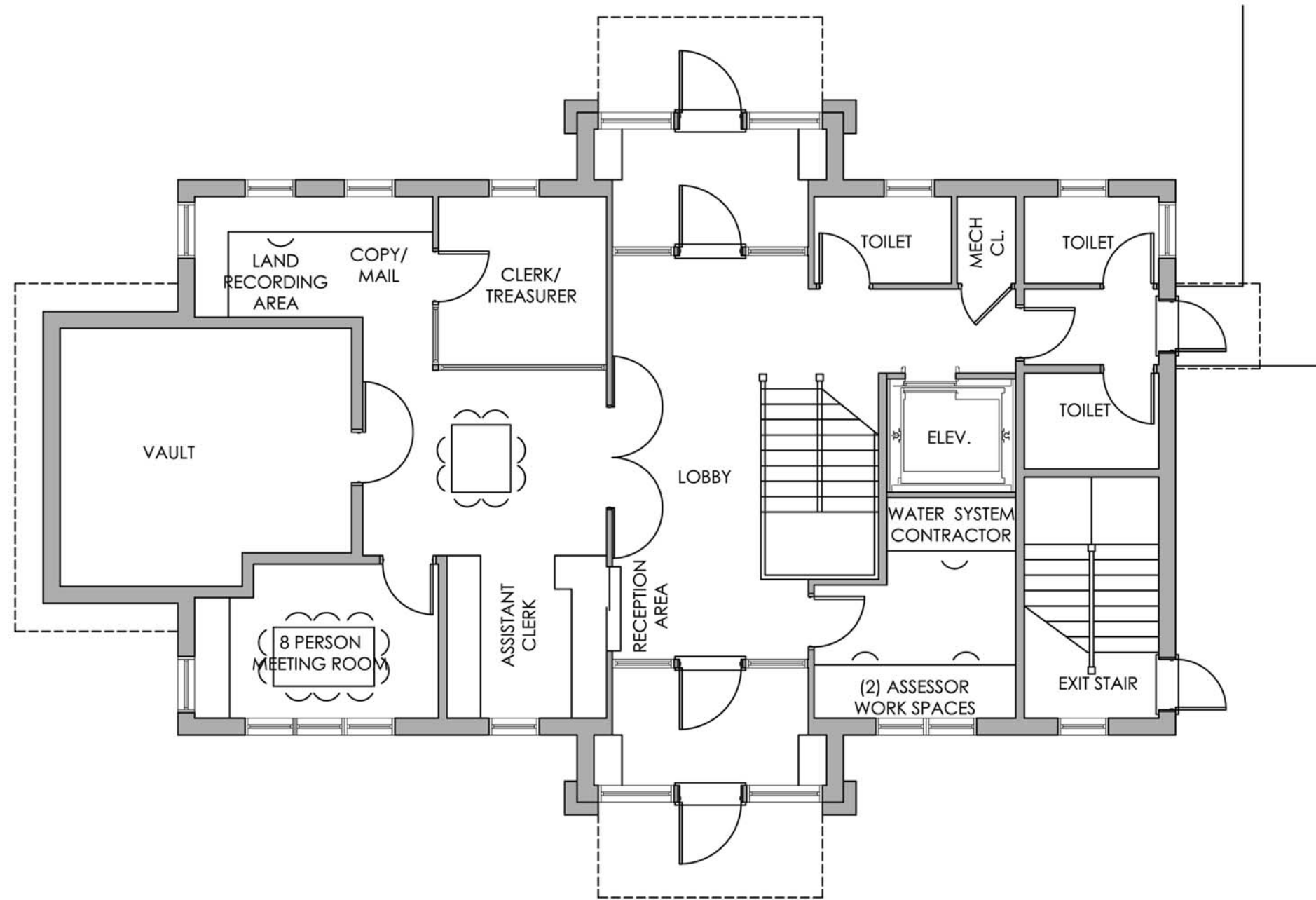
PROPOSED 1ST FLOOR PLAN 2223 GSF
